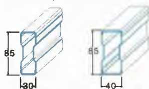
箱型橫梁 (LB) Two 'c' shaped half beam
