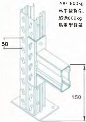
方通橫梁 (BB) Boxed beam
