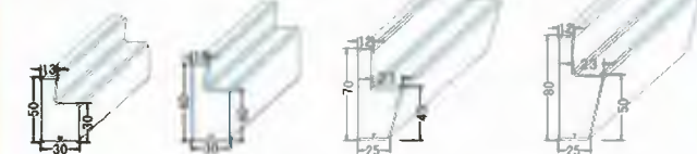
階梯橫梁 (SB) Stepped beam
