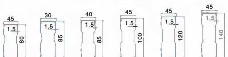
箱型橫樑截面 (LB) Double 'c' shaped half sections
